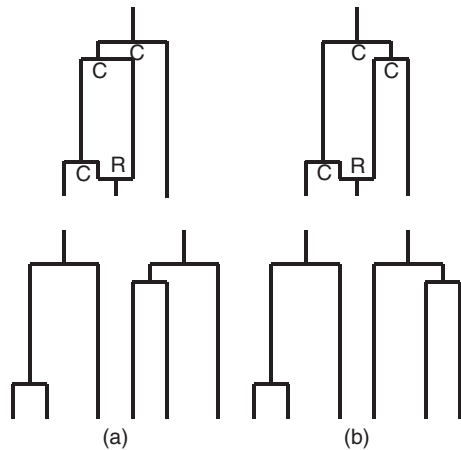
Fig. 1. Recombination graphs (Hudson, 1983) (above) and corresponding trees (below) illustrating (a) a recombination event that changes the tree length but not the topology and (b) a recombination event that changes both the tree length and the topology. In the recombination graphs, the letter C indicates coalescent events while the letter R indicates recombination events.
