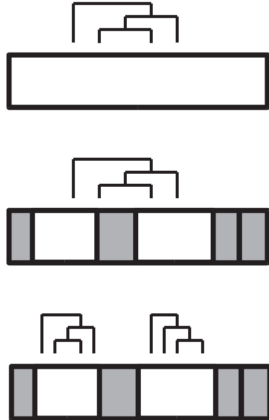
Fig. 2. Strategy for partitioning sequences according to recombination breakpoints. Full sequence (top): the entire sequence is used and described by a single tree topology and set of branch lengths, ignoring recombination breakpoints. Largest unrecombined segments, unpartitioned (middle): only codons in the largest N segments that contain no recombination breakpoints (vertical lines) are used (illustrated here by the white regions, with N = 2 ). As for the full sequence analysis, these codons are described by a single tree topology and set of branch lengths. Partitioning using largest unrecombined segments (bottom): each of the largest N segments that contain no recombination breakpoints is modelled using a separate topology and set of branch lengths.
